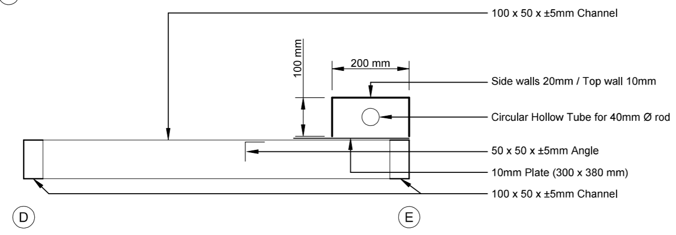
CONNECTION DETAIL - RAMP TO STRUCTURE SCALE 1:1
