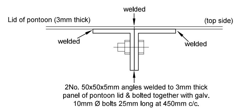
DETAIL B - FIXING DETAIL OF PONTOON LID PANELS NTS
