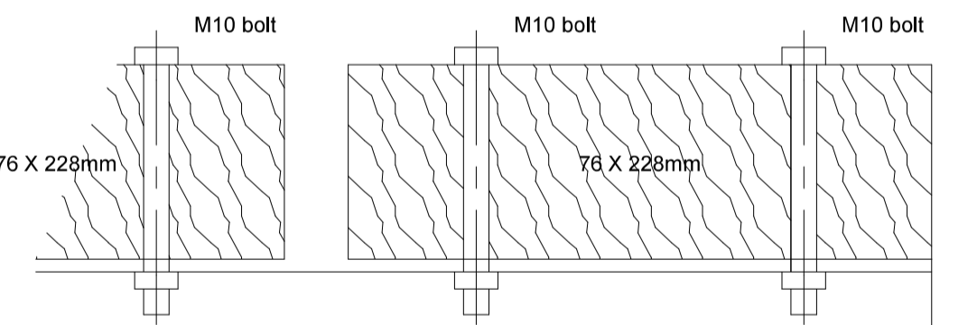
TOP VIEW - PONTOON 1:2
