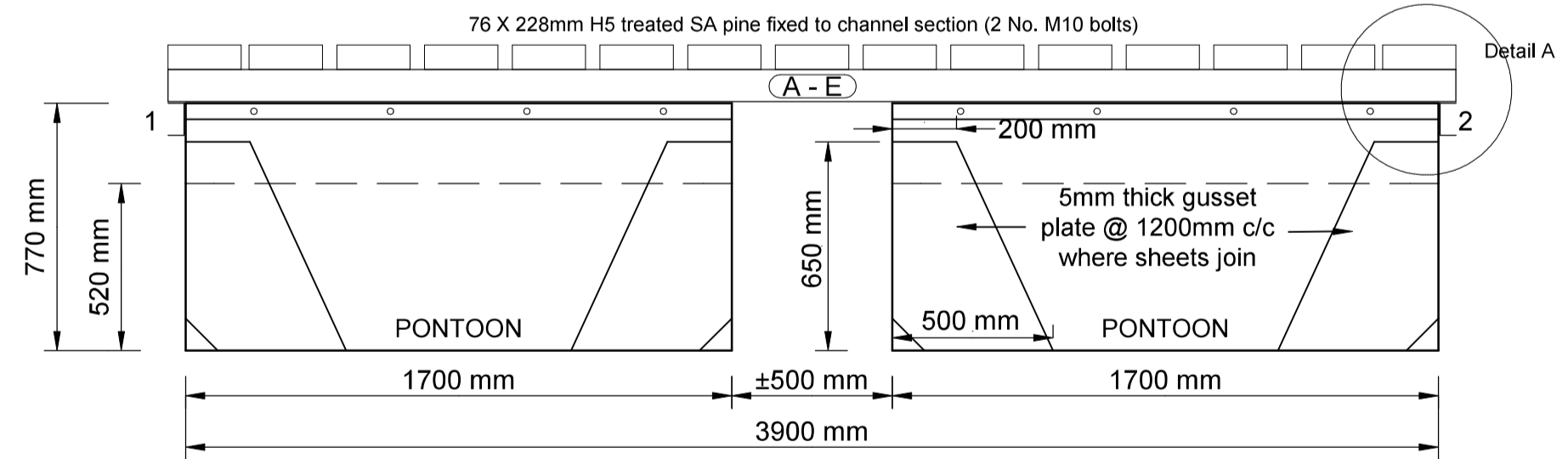
FRONT VIEW - PONTOON 1:2
