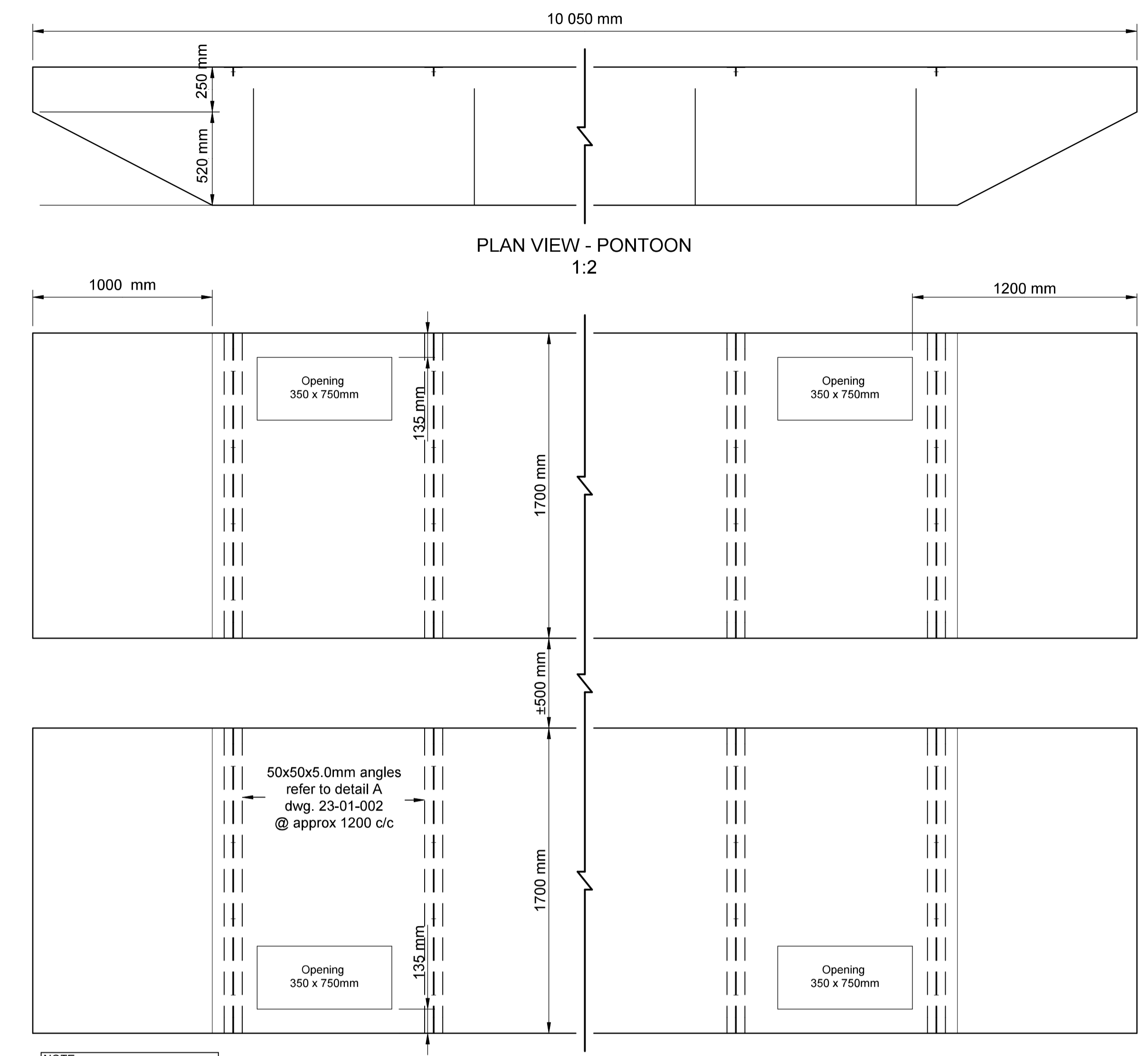
TOP VIEW - PONTOON 1:2
