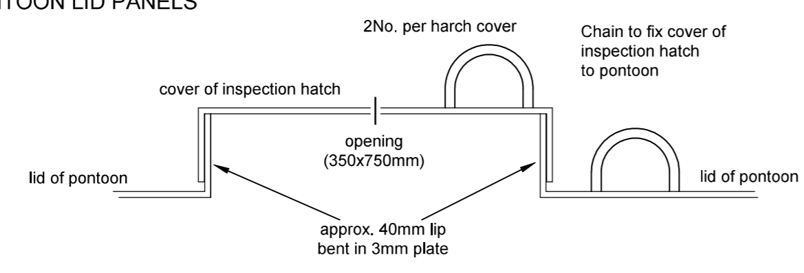
DETAIL - COVER OF INSPECTION HATCH (350X750mm) NTS
