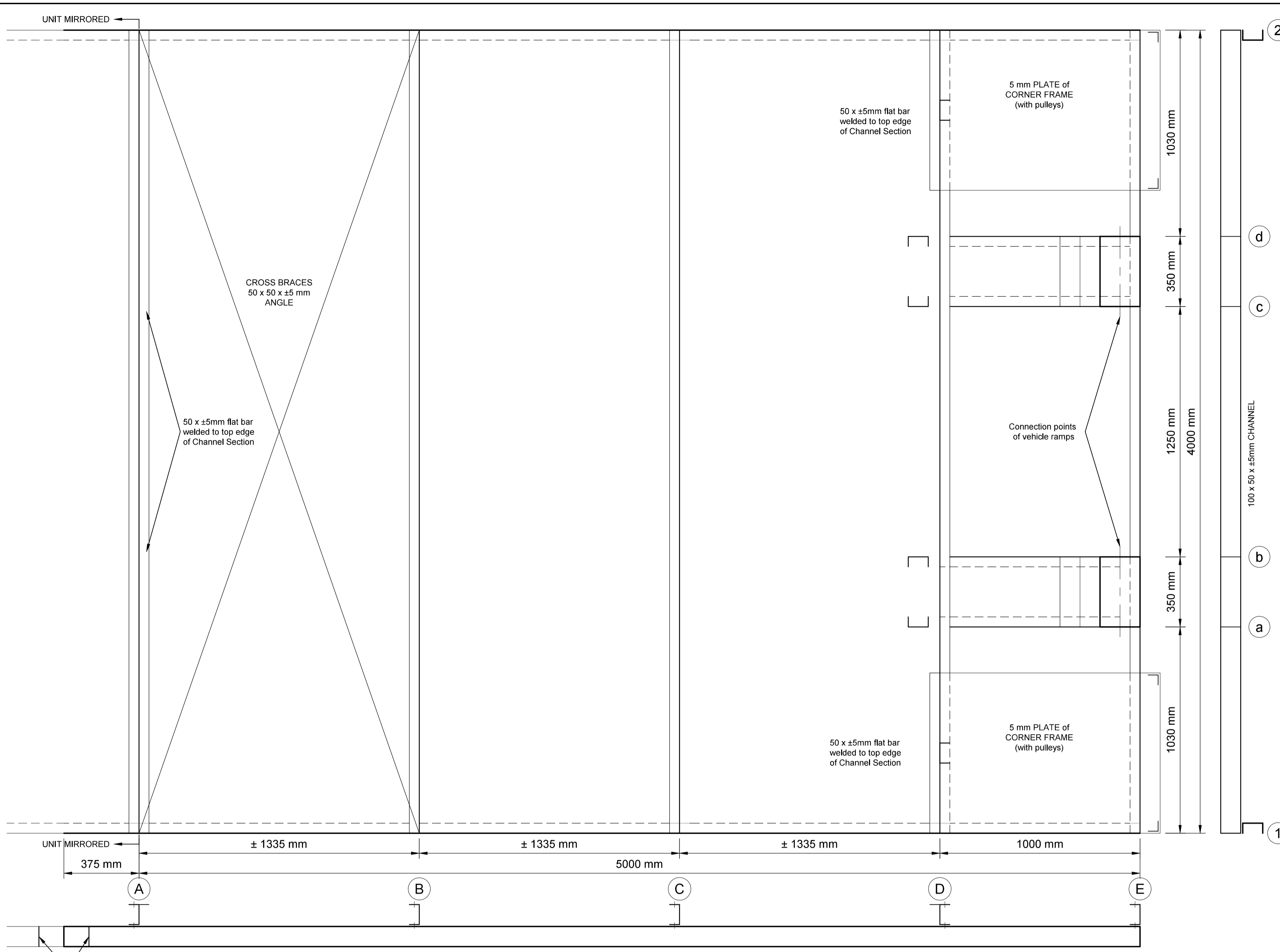
PLAN VIEW - STEEL FRAME STRUCTURE NTS
